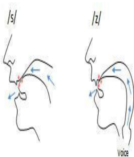
Place of Articulation : Alveolar Fricatives © Tanvir Shameem
